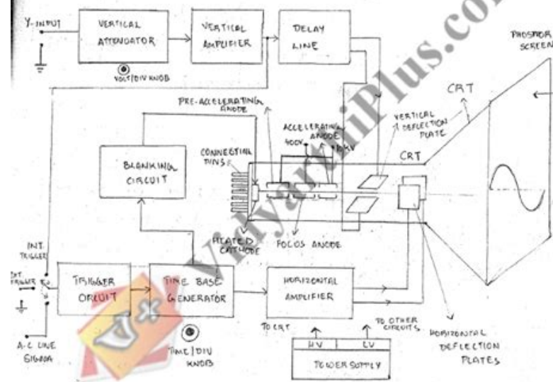
Block diagram of CRO.
